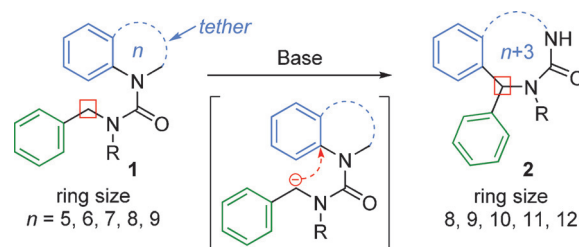
Scheme 1. Migratory ring expansion of metalated ureas.
